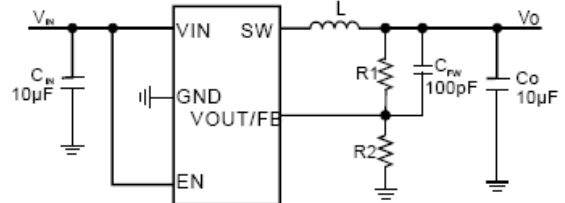
Adjustable Output Voltage
